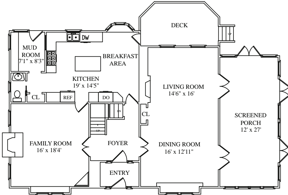
FIRST FLOOR
