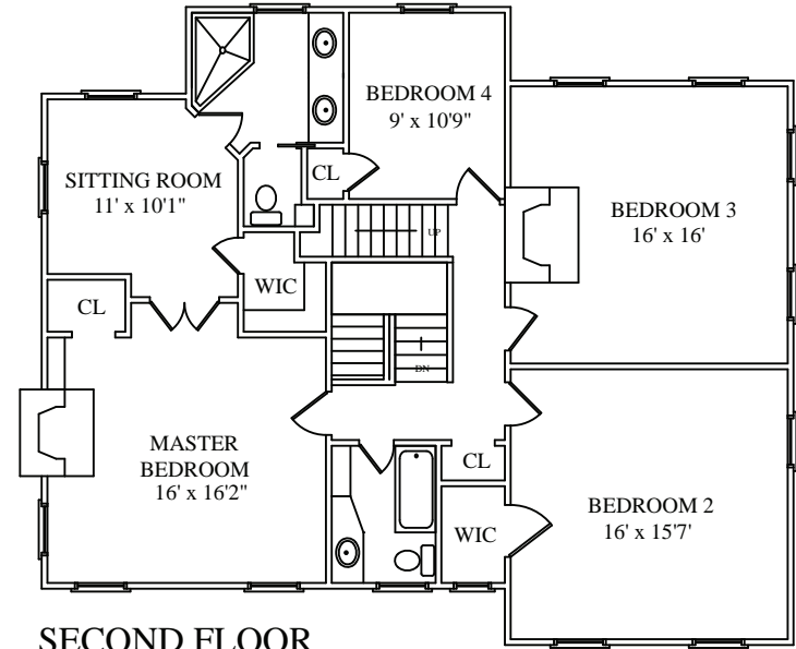
SECOND FLOOR
