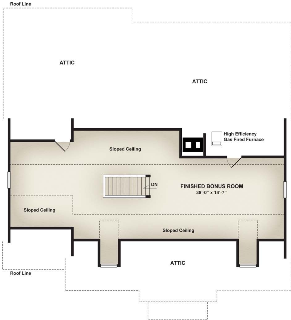
UPPER LEVEL BONUS ROOM PLAN 11 ROCKRIDGE
